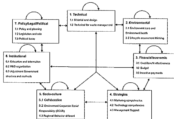
Fig.1 ANP construction of influence factor for management of flexible packaging waste
